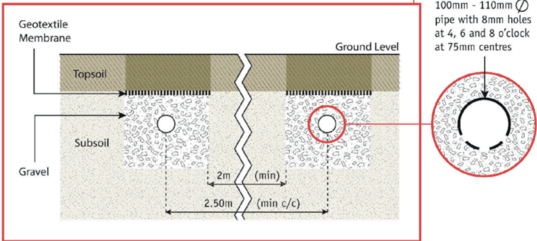
FIGURE 7.1. PLAN AND SECTION OF LAYOUT OF SEPTIC TANK SYSTEM.
